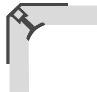
Innenecke 7-10 mm
